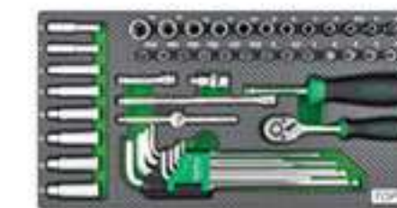
ITEM NO. CONTENTS 6 (SET) GEA5004 13 BAEA0804-0814 1/4" Dr. 6PT Flank Sockets 4, 4.5, 5, 5.5, 6, 7, 8, 9, 10, 11, 12, 13, 14 mm 8 BAE0806-0813 1/4" Dr. 6PT Flank Deep Sockets 6, 7, 8, 9, 10, 11, 12, 13 mm 3 BCDA0803-0808 1/4" Dr. Hex Bit Sockets 3, 4, 5, 6, 8 mm 3 BCCA0803-0808 1/4" Dr. Slotted Bit Sockets 3, 5.5, 8 mm 3 BCAA08P0-08P2 1/4" Dr. Phillips Bit Sockets PH0, PH1, PH2 3 BCBA08P0-08P2 1/4" Dr. Pozzi Bit Sockets PZ0, PZ1, PZ2 1 CAIP0816 1/4" Dr. Spinner Handle 1 CTCK0811 1/4" Dr. Sliding T-Handle 1 CAHA0840 1/4" Dr. Universal Joint 2 CAAA0802 & 0806 1/4" Dr. Extension Bar - 2" & 6" (L) 1 CJB0815 1/4" Dr. 72 Teeth Reversible Ratchet Handle with Quick Release 1 GSN-09EB Extra Long Ball Point Hex Key Wrench Set 1.5, 2, 2.5, 3, 4, 5, 6, 8, 10 mm
